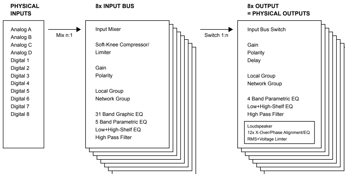
Figure 1.1.: Signal Path
